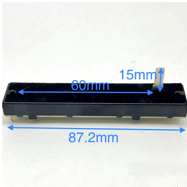
Fader 20K X2 88mm course 60mm type piste Vestax PMC-280
