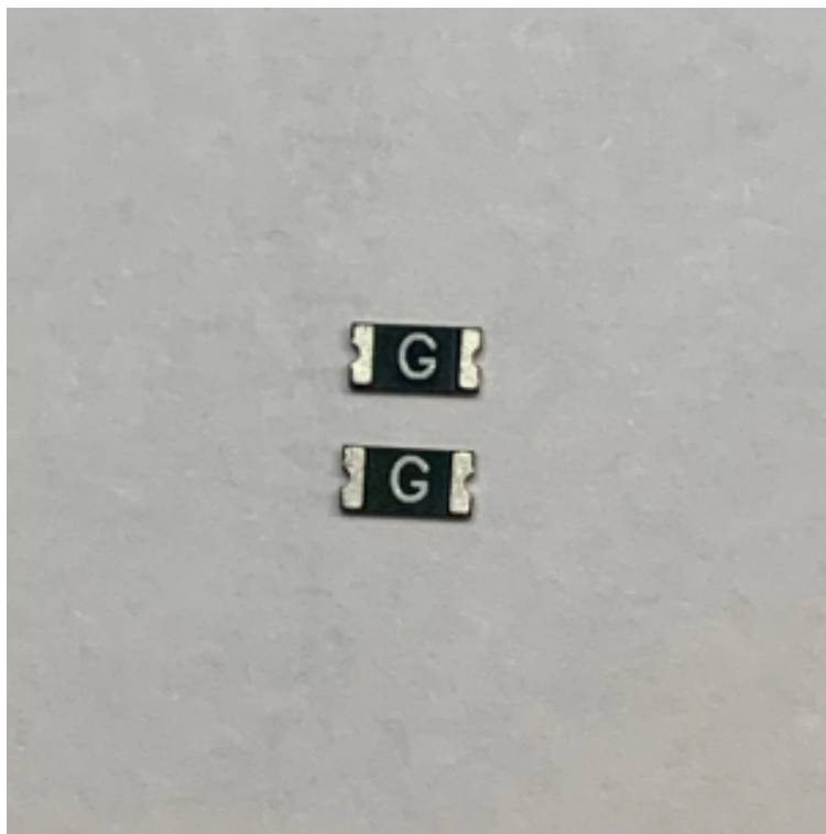
Fusible G 750mA 63V SMD boitier 1206
